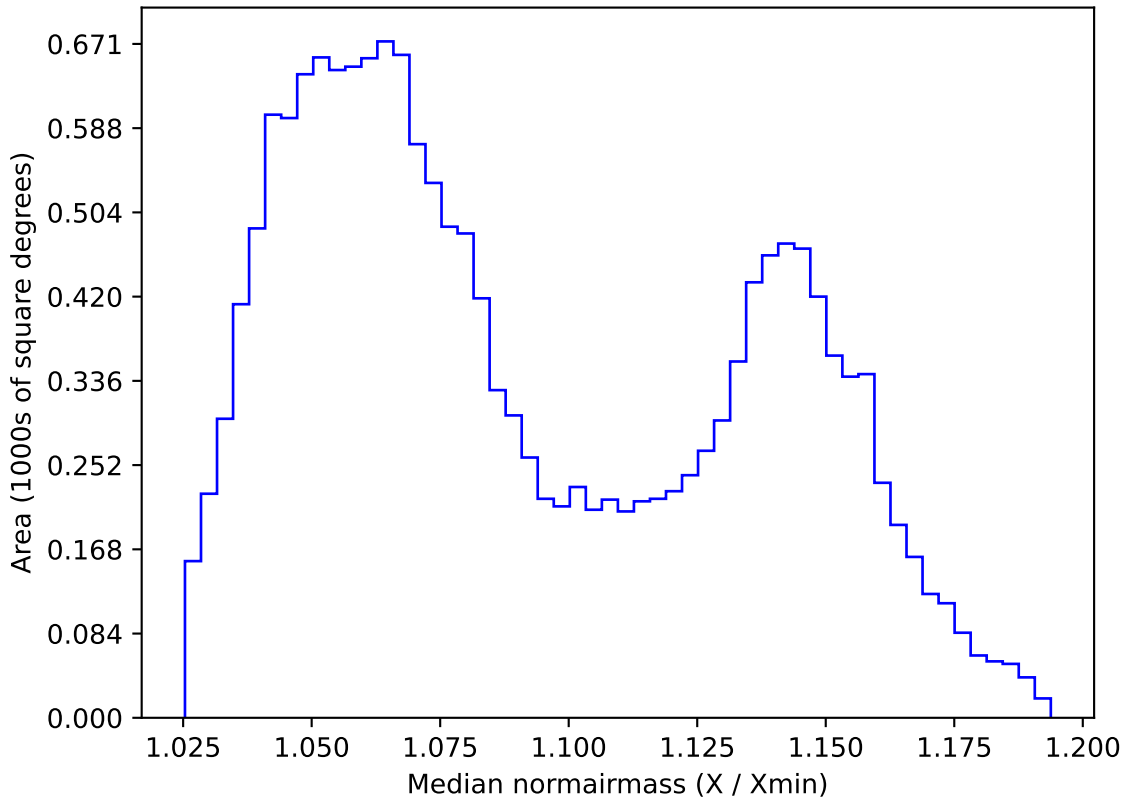
too_elab_r32_d3_ugrizy_v3.4_10yrs WFD y band: Median normairmass
