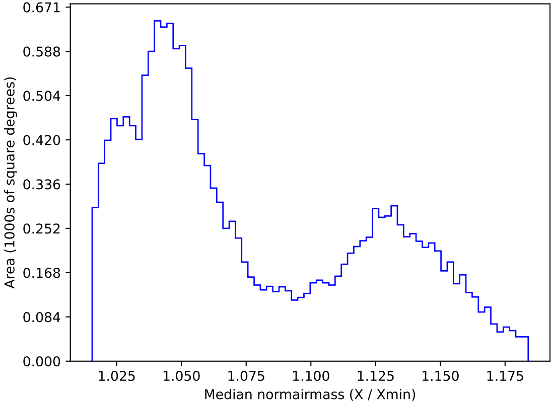
too_elab_r32_d3_ugrizy_v3.4_10yrs WFD r band: Median normairmass
