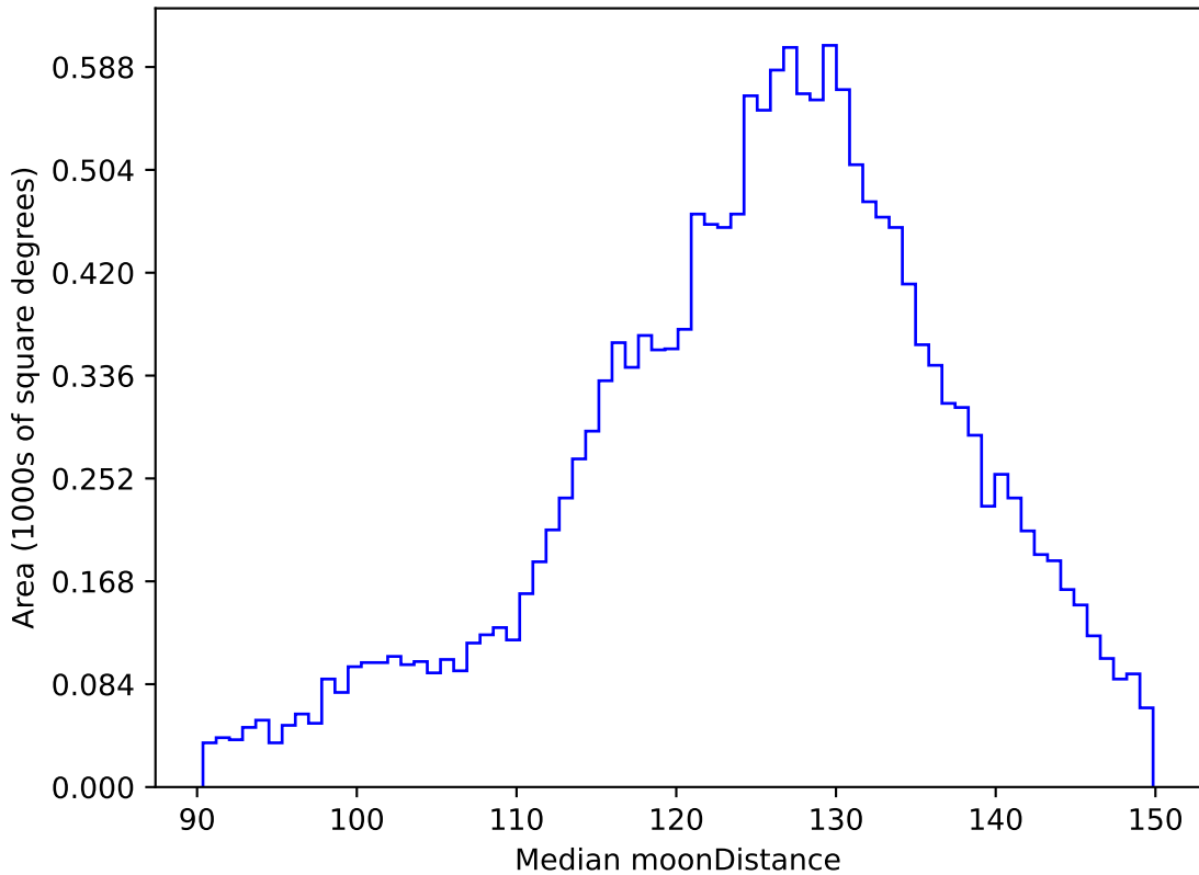
too_elab_r32_d3_ugrizy_v3.4_10yrs WFD u band: Median moonDistance
