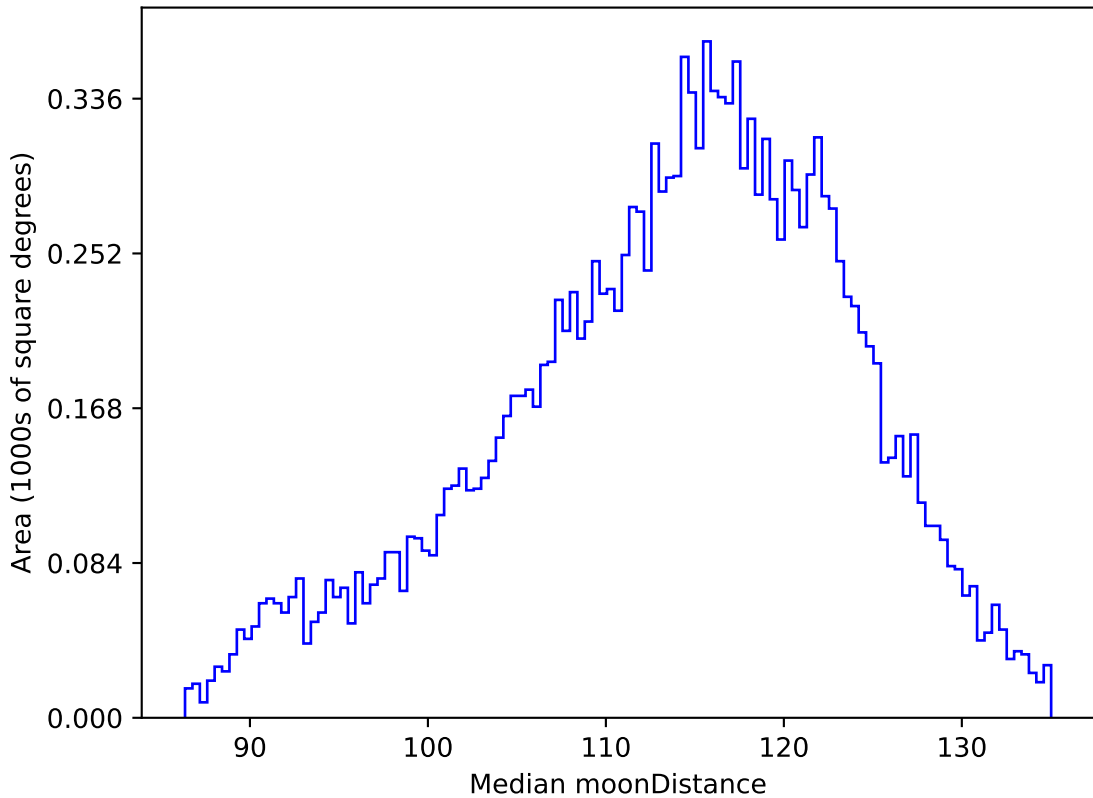
too_elab_r32_d3_ugrizy_v3.4_10yrs WFD g band: Median moonDistance
