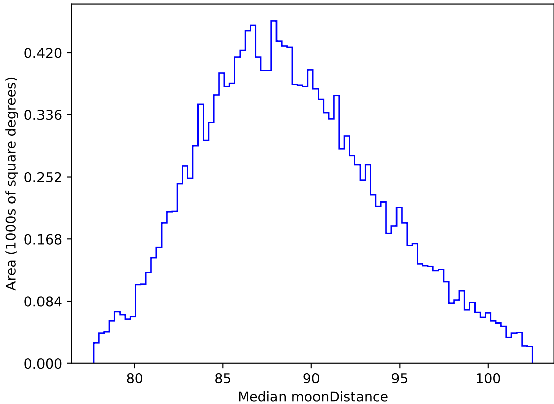
too_elab_r32_d3_ugrizy_v3.4_10yrs WFD all bands: Median moonDistance
