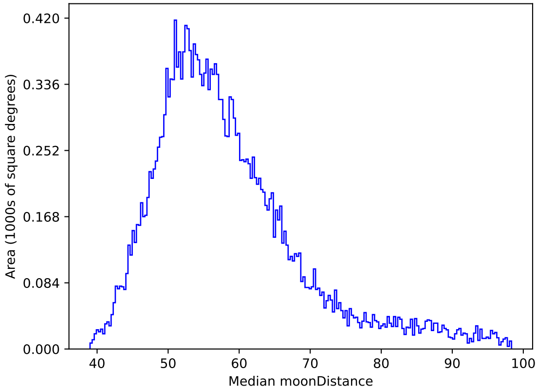
too_elab_r32_d3_ugrizy_v3.4_10yrs All sky y band: Median moonDistance
