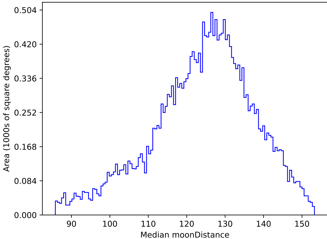
too_elab_r32_d3_ugrizy_v3.4_10yrs All sky u band: Median moonDistance
