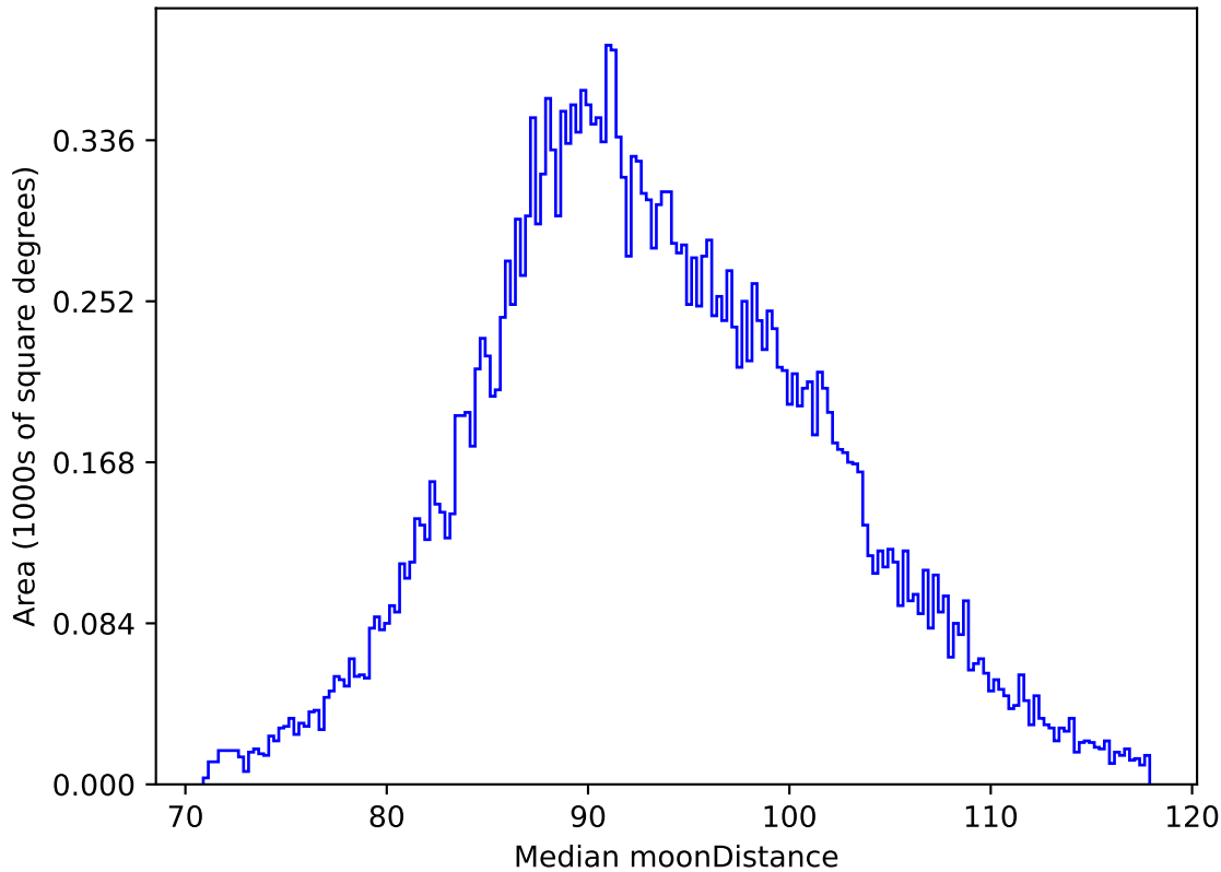
too_elab_r32_d3_ugrizy_v3.4_10yrs All sky i band: Median moonDistance
