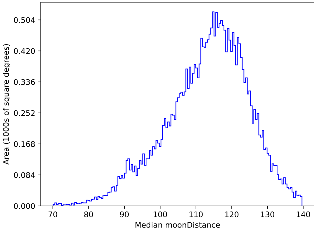
too_elab_r32_d3_ugrizy_v3.4_10yrs All sky g band: Median moonDistance
