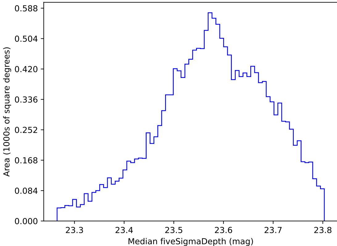
too_elab_r32_d3_ugrizy_v3.4_10yrs WFD i band: Median fiveSigmaDepth
