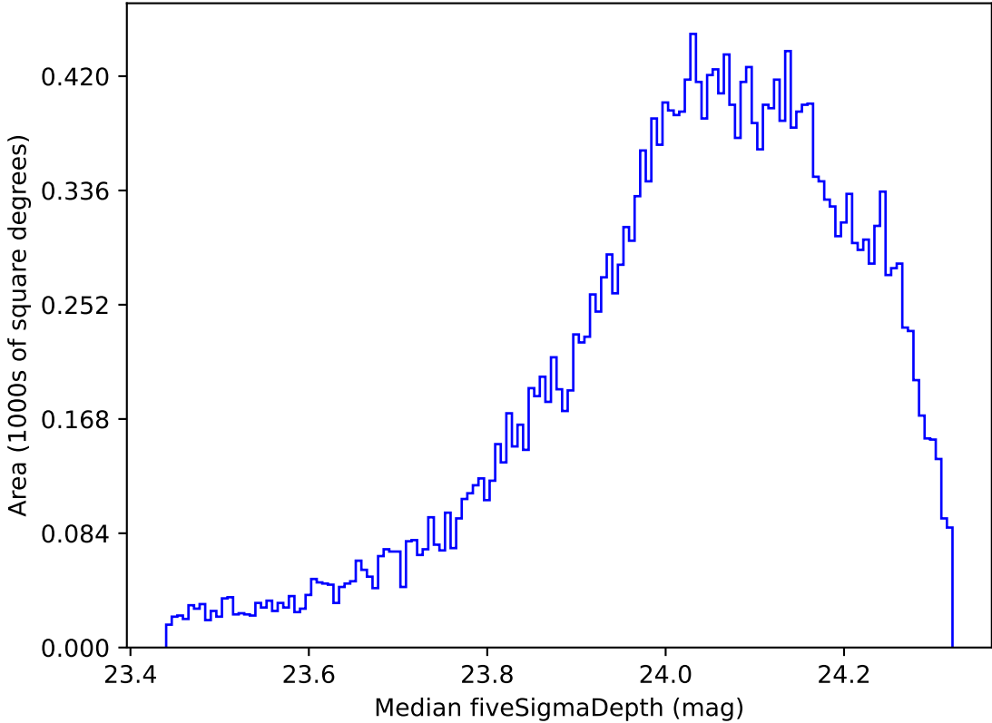
too_elab_r32_d3_ugrizy_v3.4_10yrs All sky r band: Median fiveSigmaDepth
