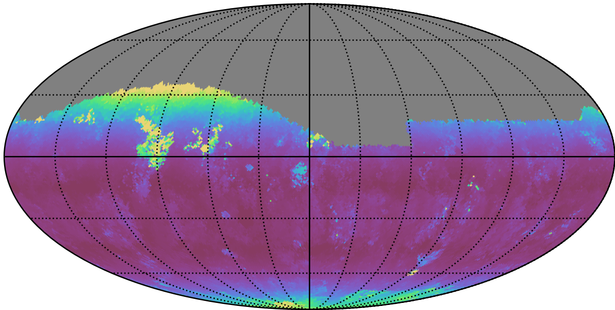
too_elab_r32_d3_ugrizy_v3.4_10yrs Yr 1 z band: Median airmass
