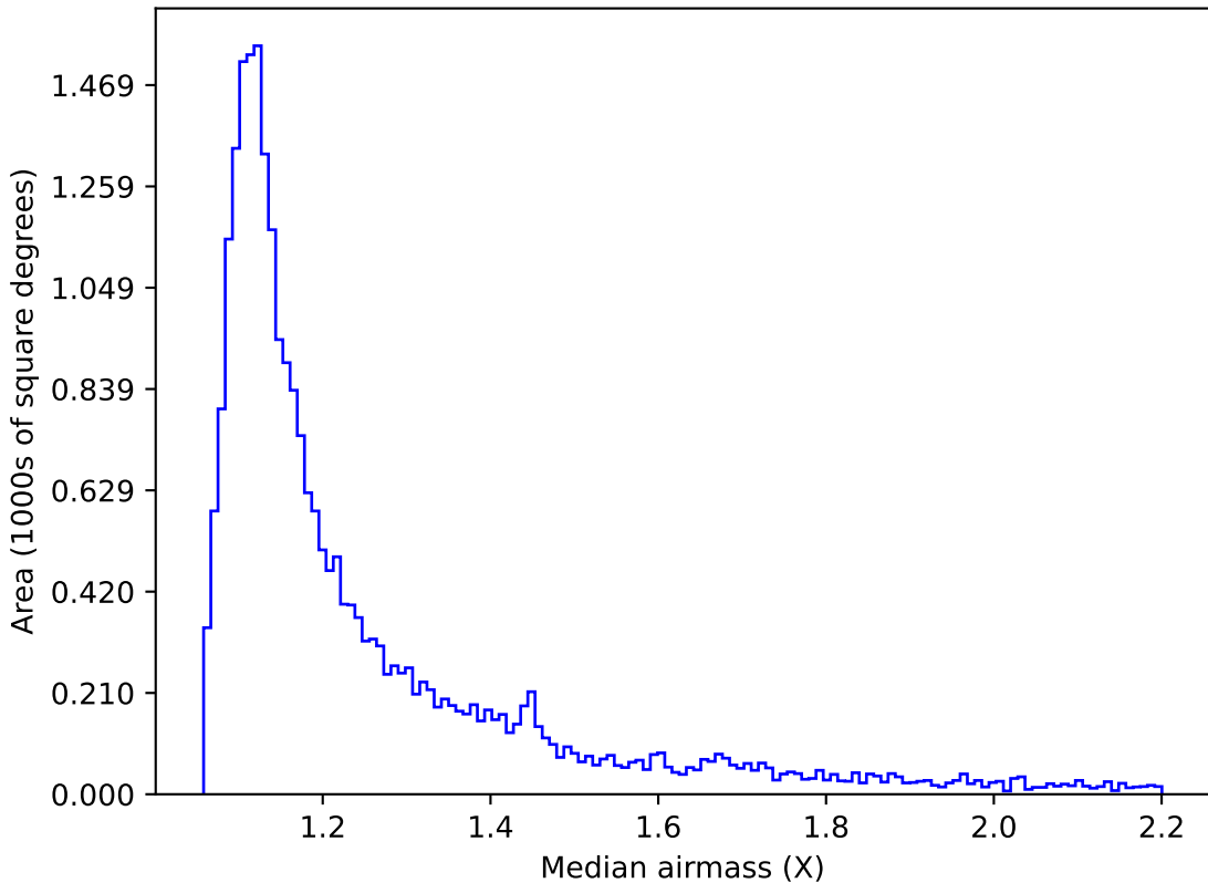
too_elab_r32_d3_ugrizy_v3.4_10yrs Yr 1 z band: Median airmass
