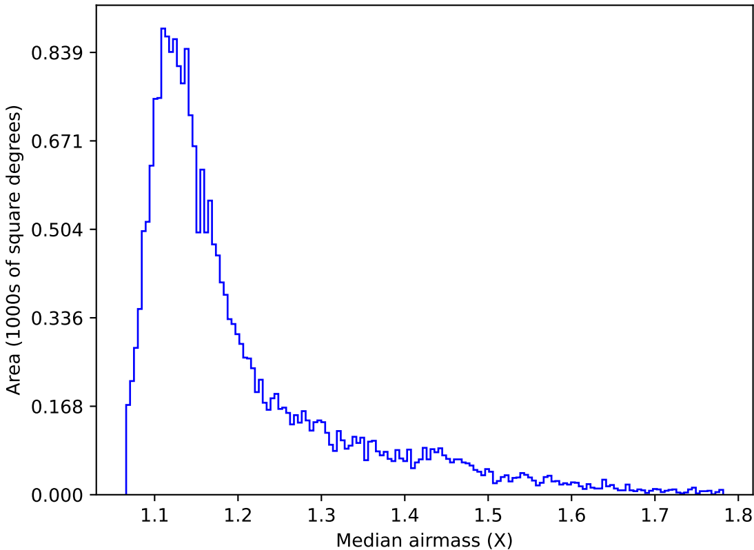
too_elab_r32_d3_ugrizy_v3.4_10yrs Yr 1 y band: Median airmass
