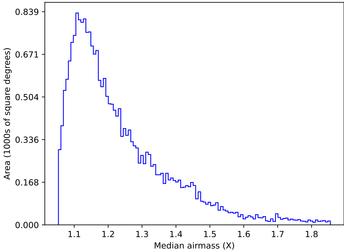
too_elab_r32_d3_ugrizy_v3.4_10yrs Yr 1 u band: Median airmass
