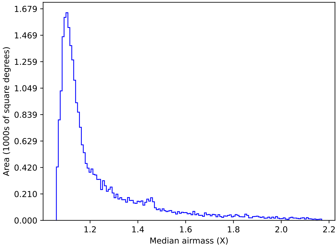
too_elab_r32_d3_ugrizy_v3.4_10yrs Yr 1 i band: Median airmass
