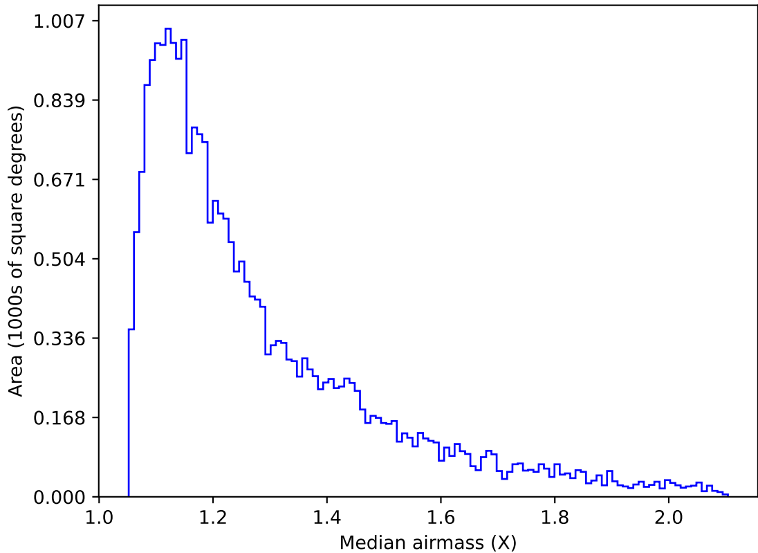
too_elab_r32_d3_ugrizy_v3.4_10yrs Yr 1 g band: Median airmass
