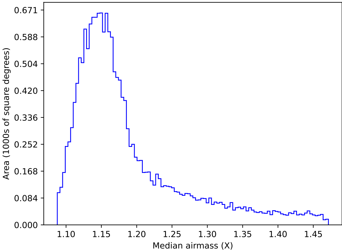
too_elab_r32_d3_ugrizy_v3.4_10yrs WFD z band: Median airmass
