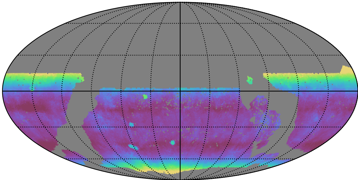
too_elab_r32_d3_ugrizy_v3.4_10yrs WFD y band: Median airmass
