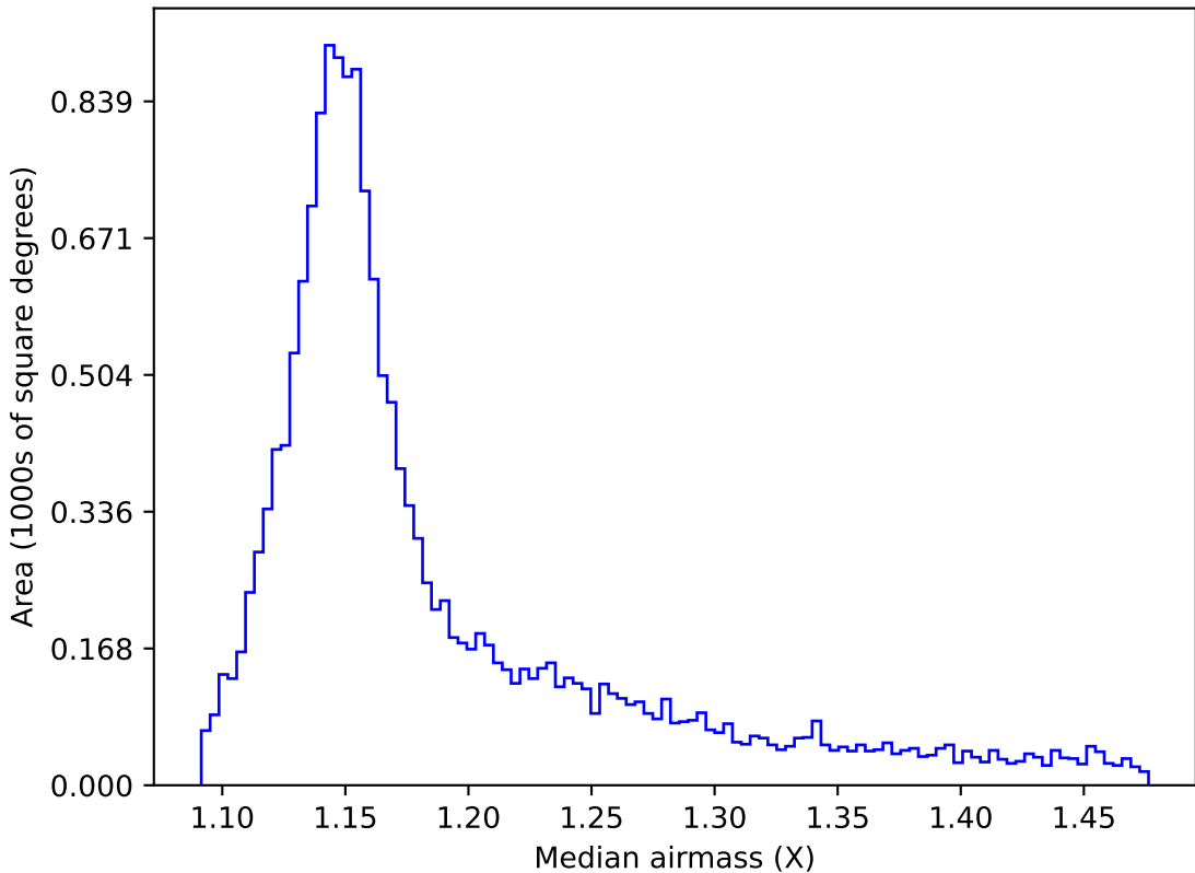
too_elab_r32_d3_ugrizy_v3.4_10yrs WFD y band: Median airmass
