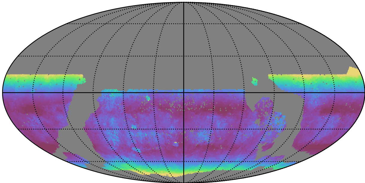
too_elab_r32_d3_ugrizy_v3.4_10yrs WFD u band: Median airmass
