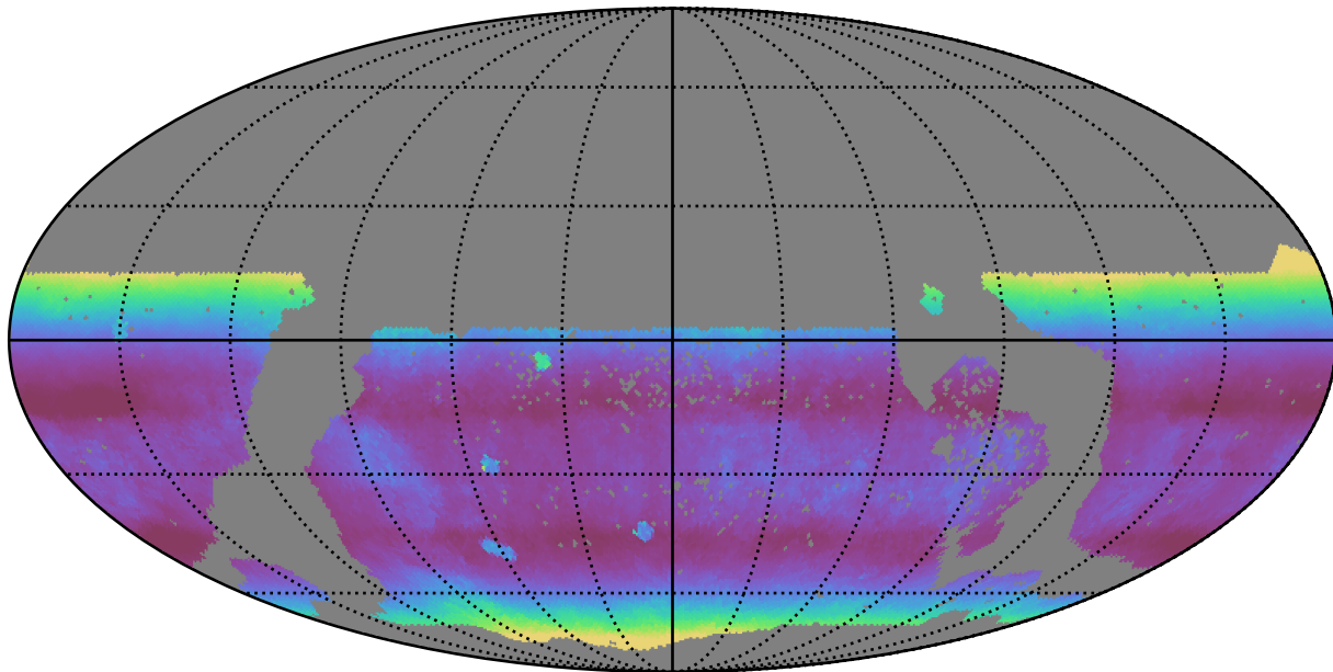
too_elab_r32_d3_ugrizy_v3.4_10yrs WFD r band: Median airmass
