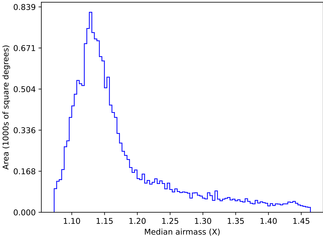
too_elab_r32_d3_ugrizy_v3.4_10yrs WFD r band: Median airmass
