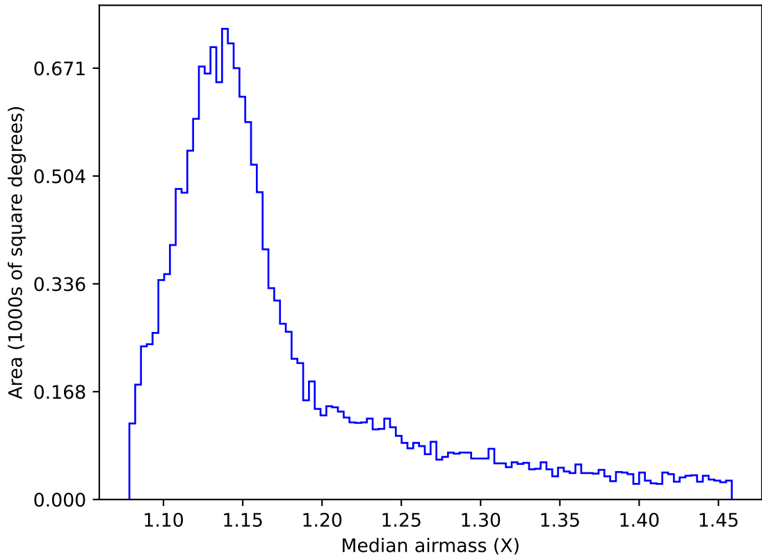
too_elab_r32_d3_ugrizy_v3.4_10yrs WFD i band: Median airmass
