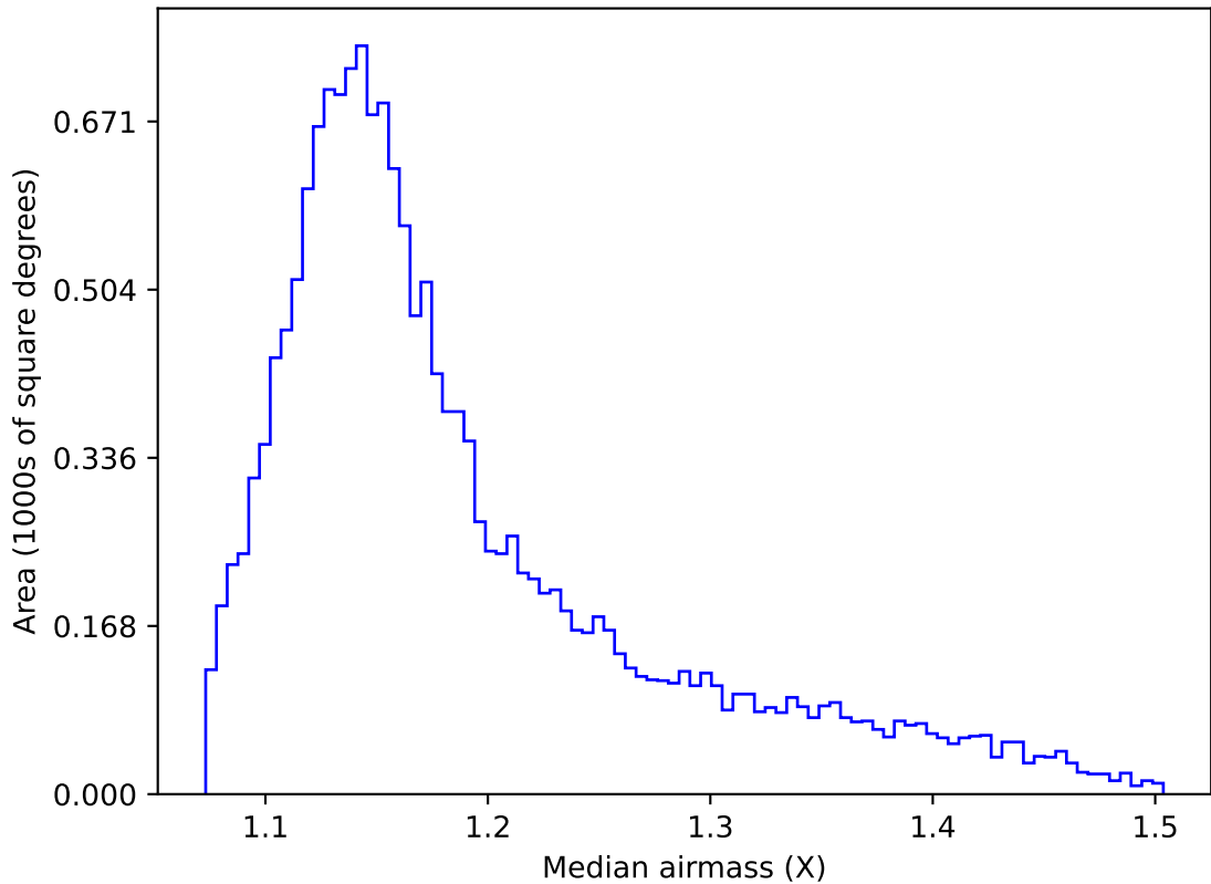
too_elab_r32_d3_ugrizy_v3.4_10yrs WFD g band: Median airmass
