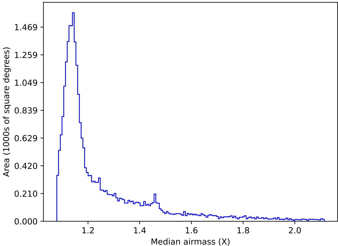
too_elab_r32_d3_ugrizy_v3.4_10yrs All sky i band: Median airmass
