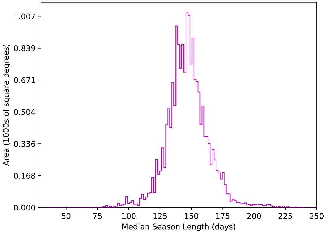
too_elab_r32_d3_ugrizy_v3.4_10yrs WFD z band: Median Season Length
