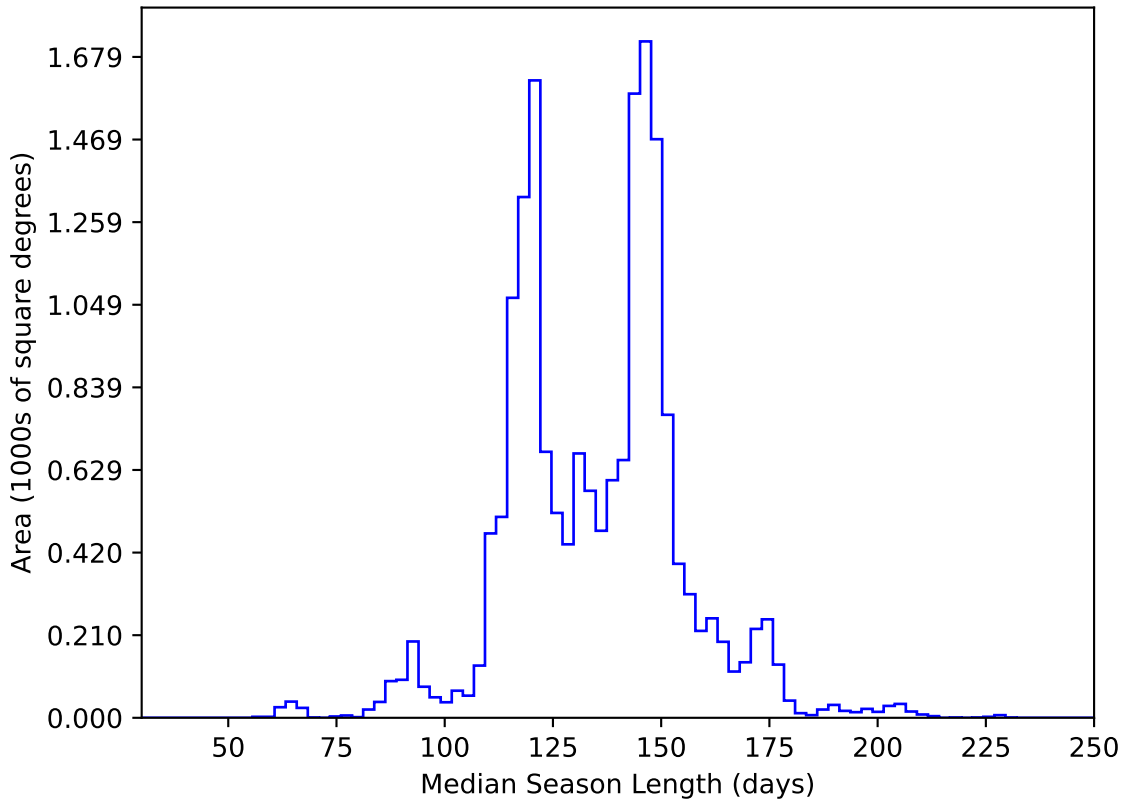
too_elab_r32_d3_ugrizy_v3.4_10yrs WFD y band: Median Season Length
