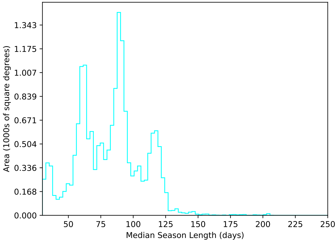
too_elab_r32_d3_ugrizy_v3.4_10yrs WFD u band: Median Season Length
