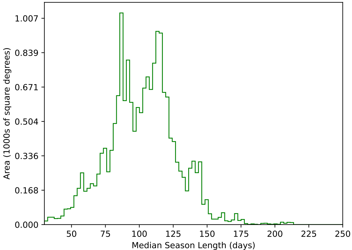
too_elab_r32_d3_ugrizy_v3.4_10yrs WFD g band: Median Season Length
