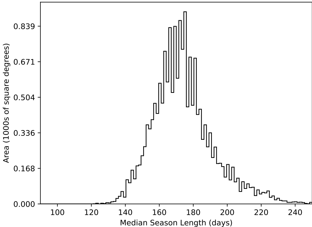
too_elab_r32_d3_ugrizy_v3.4_10yrs WFD all bands: Median Season Length
