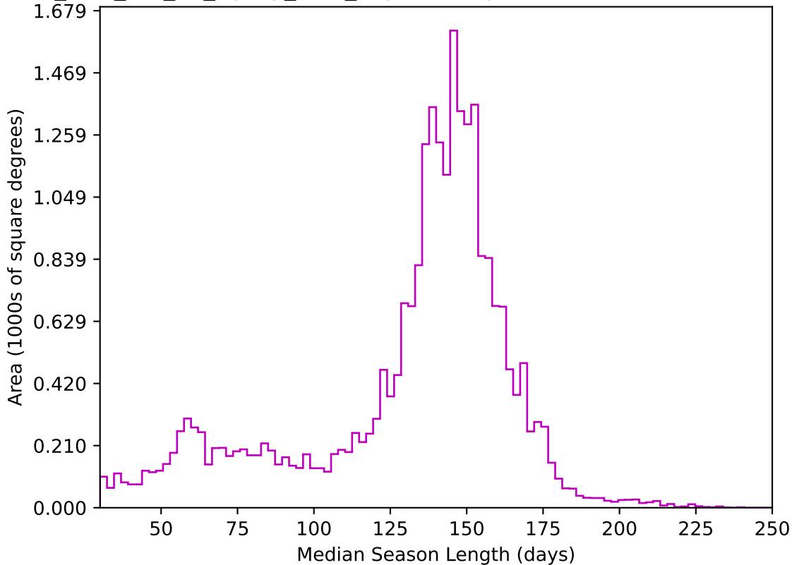
too_elab_r32_d3_ugrizy_v3.4_10yrs All sky z band: Median Season Length
