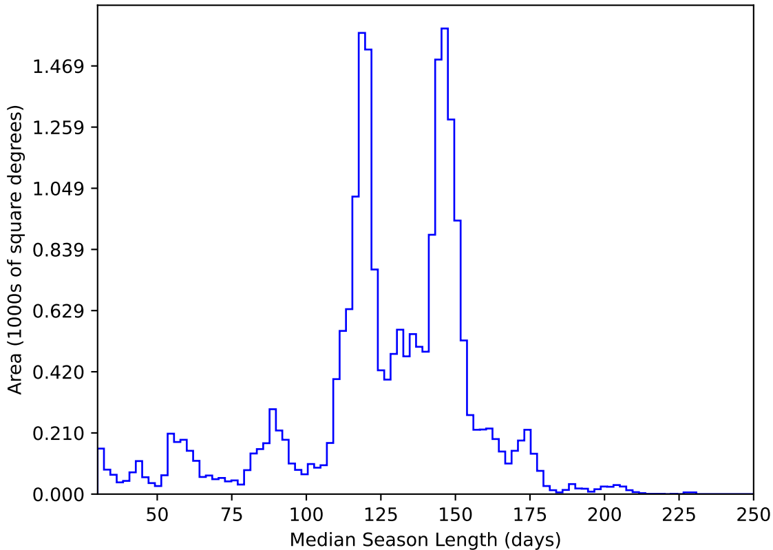
too_elab_r32_d3_ugrizy_v3.4_10yrs All sky y band: Median Season Length
