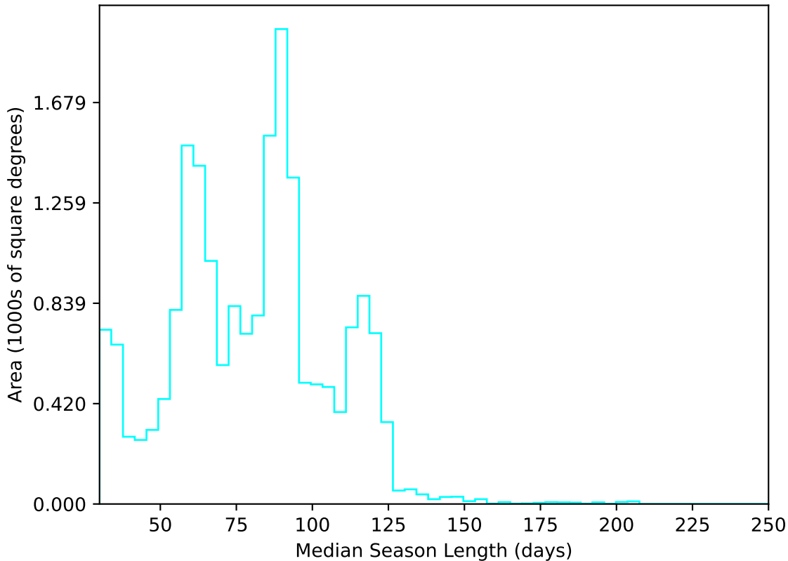
too_elab_r32_d3_ugrizy_v3.4_10yrs All sky u band: Median Season Length
