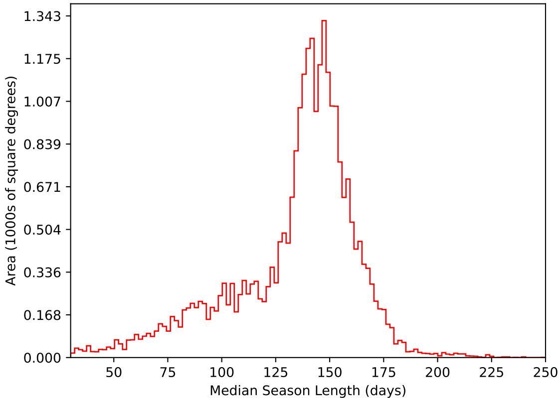
too_elab_r32_d3_ugrizy_v3.4_10yrs All sky i band: Median Season Length
