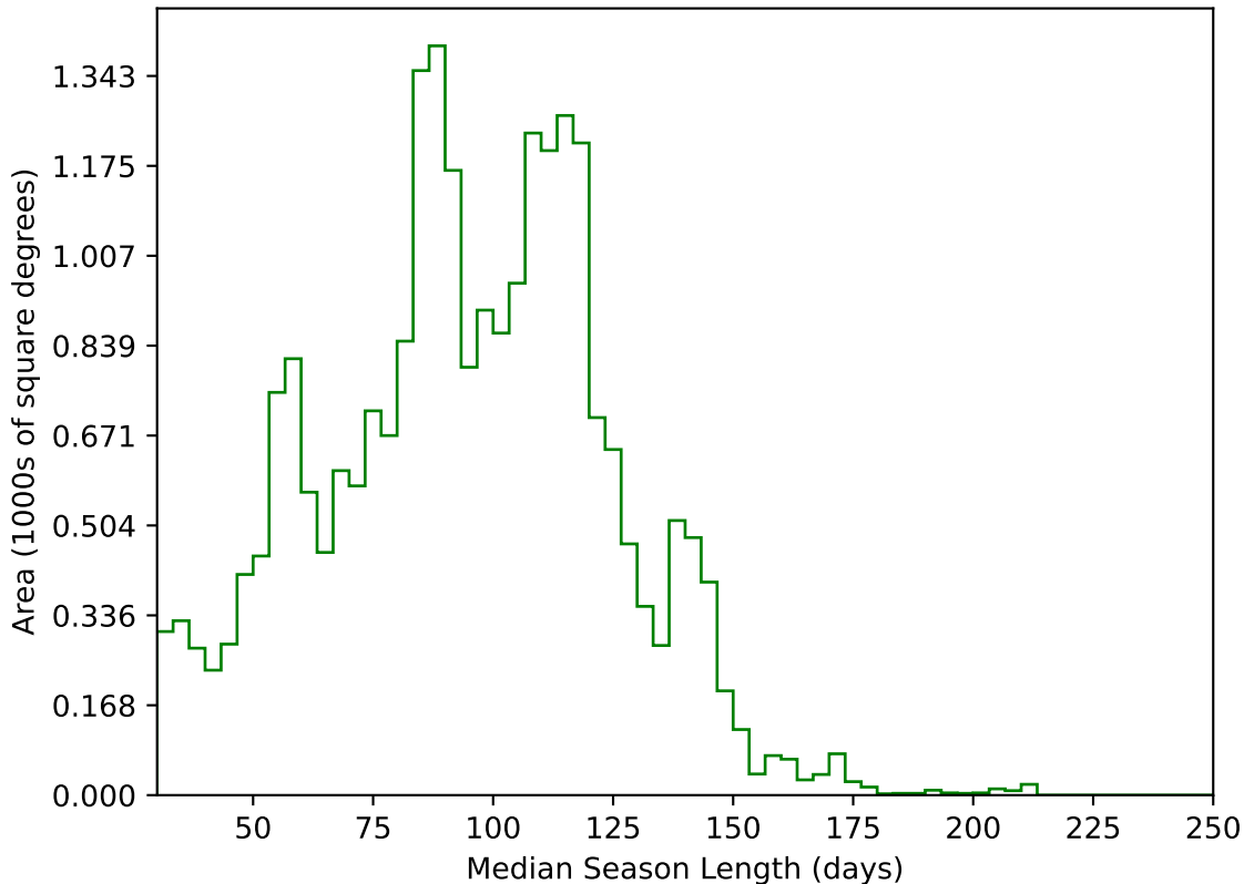
too_elab_r32_d3_ugrizy_v3.4_10yrs All sky g band: Median Season Length
