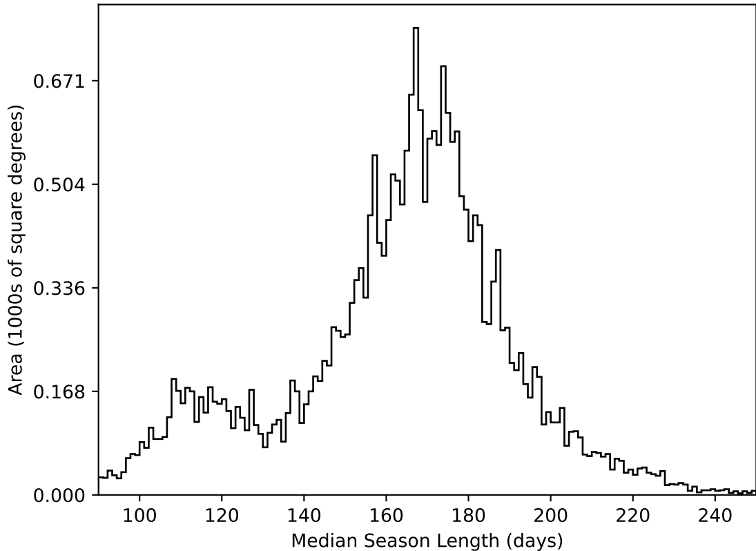
too_elab_r32_d3_ugrizy_v3.4_10yrs All sky all bands: Median Season Length
