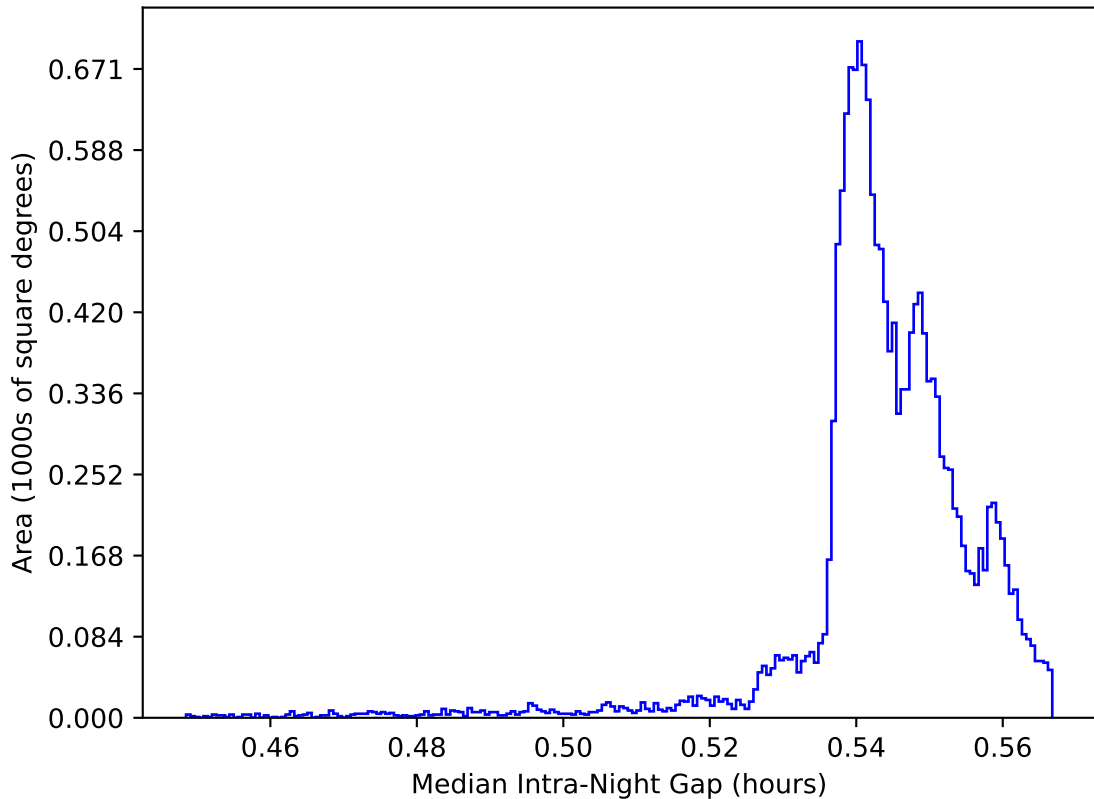
too_elab_r32_d3_ugrizy_v3.4_10yrs WFD: Median Intra-Night Gap
