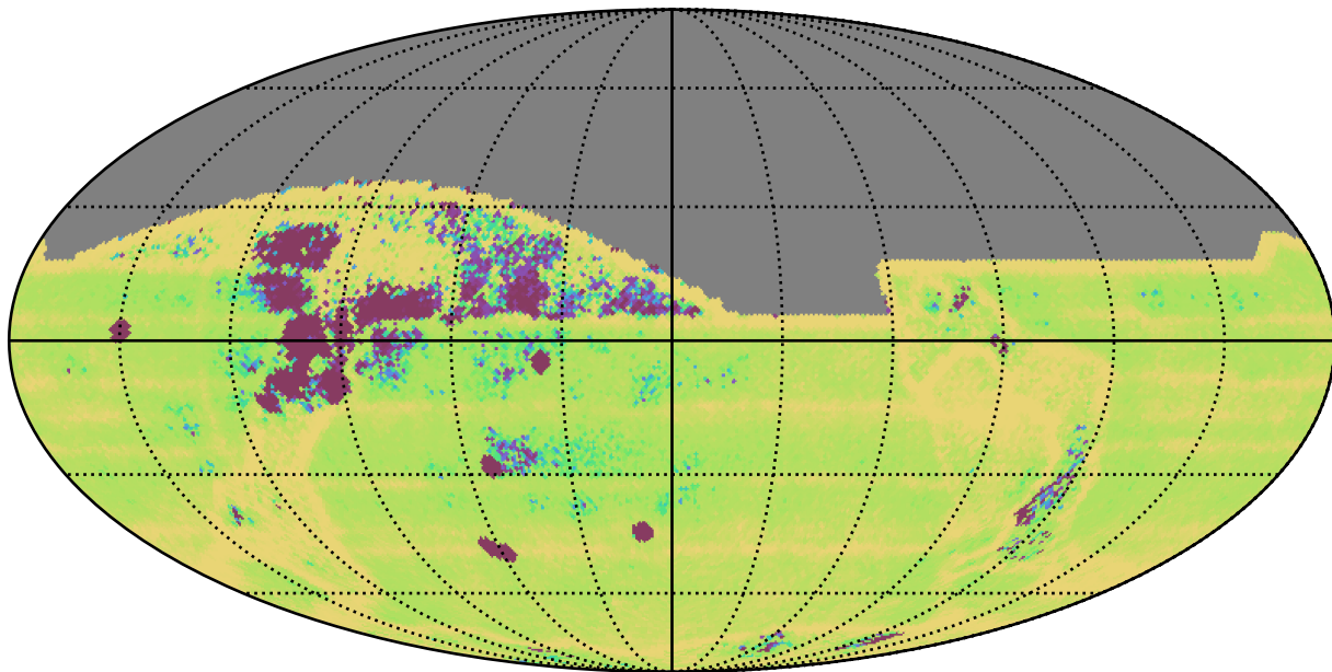
too_elab_r32_d3_ugrizy_v3.4_10yrs All sky: Median Intra-Night Gap
