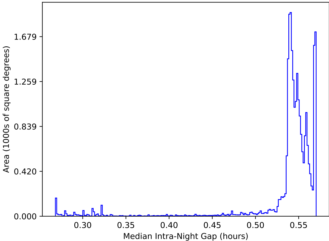
too_elab_r32_d3_ugrizy_v3.4_10yrs All sky: Median Intra-Night Gap
