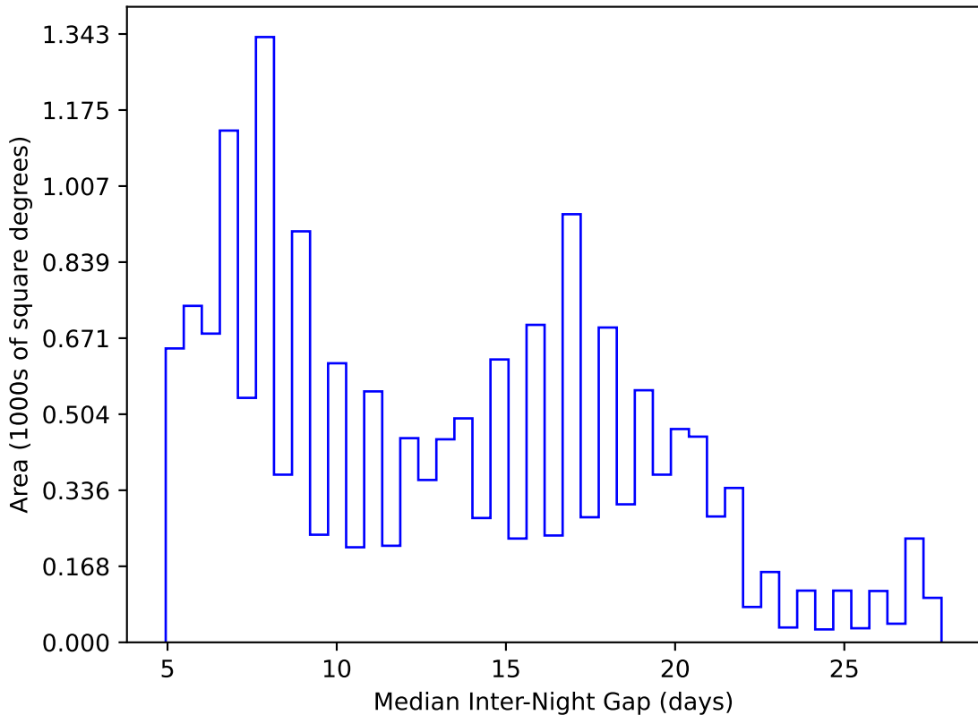
too_elab_r32_d3_ugrizy_v3.4_10yrs WFD y band: Median Inter-Night Gap
