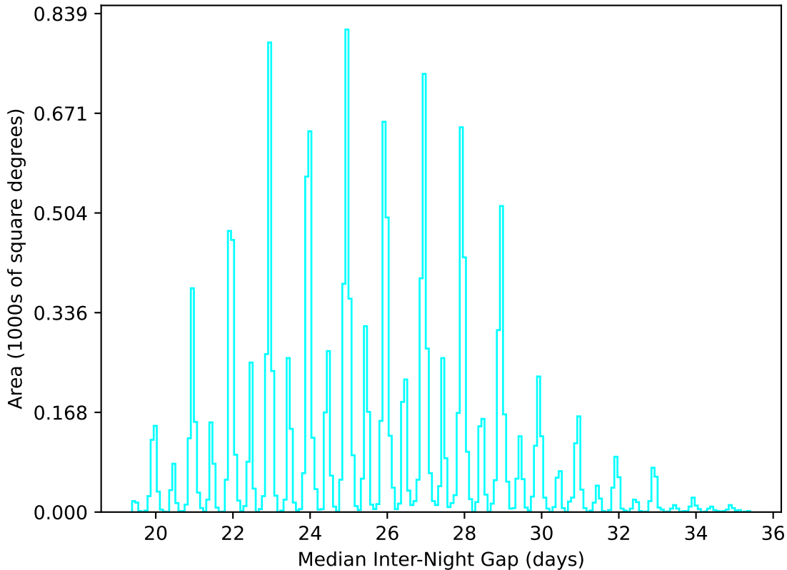
too_elab_r32_d3_ugrizy_v3.4_10yrs WFD u band: Median Inter-Night Gap
