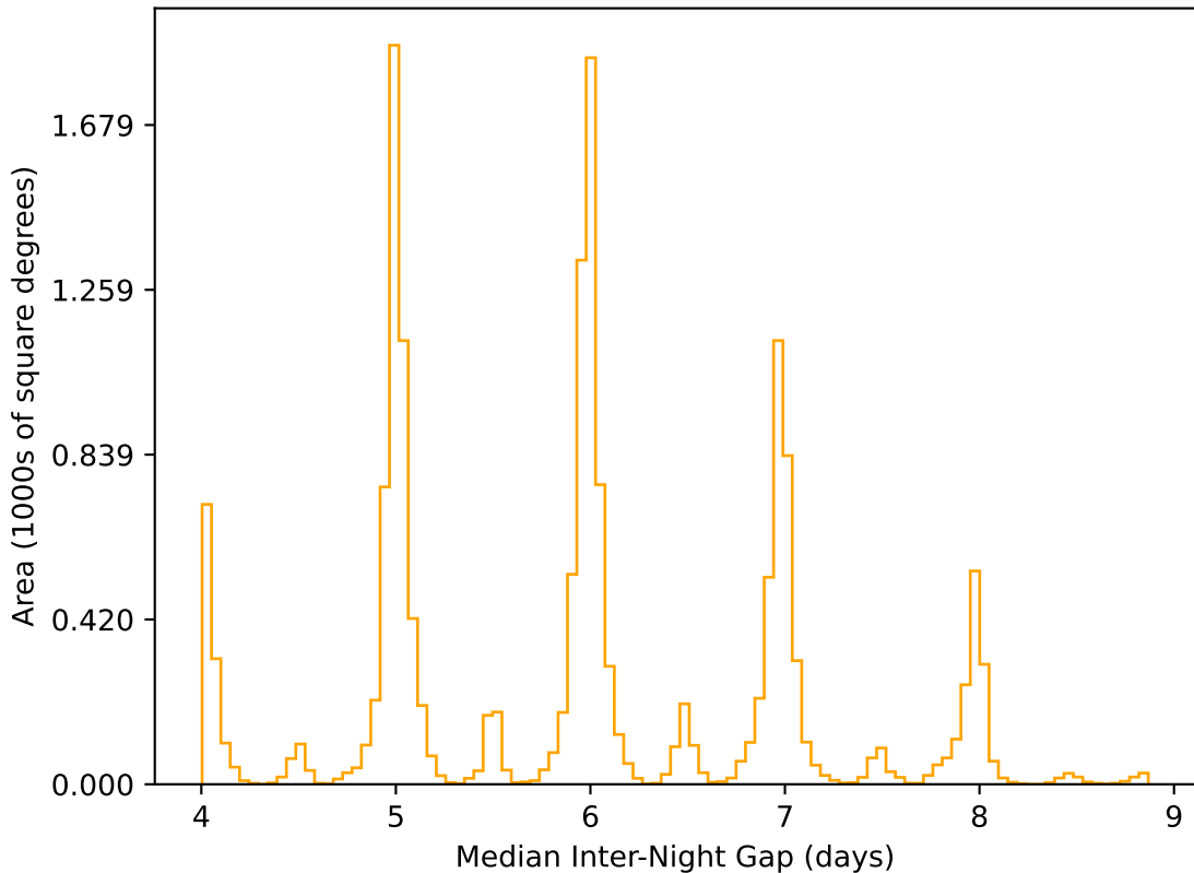
too_elab_r32_d3_ugrizy_v3.4_10yrs WFD r band: Median Inter-Night Gap
