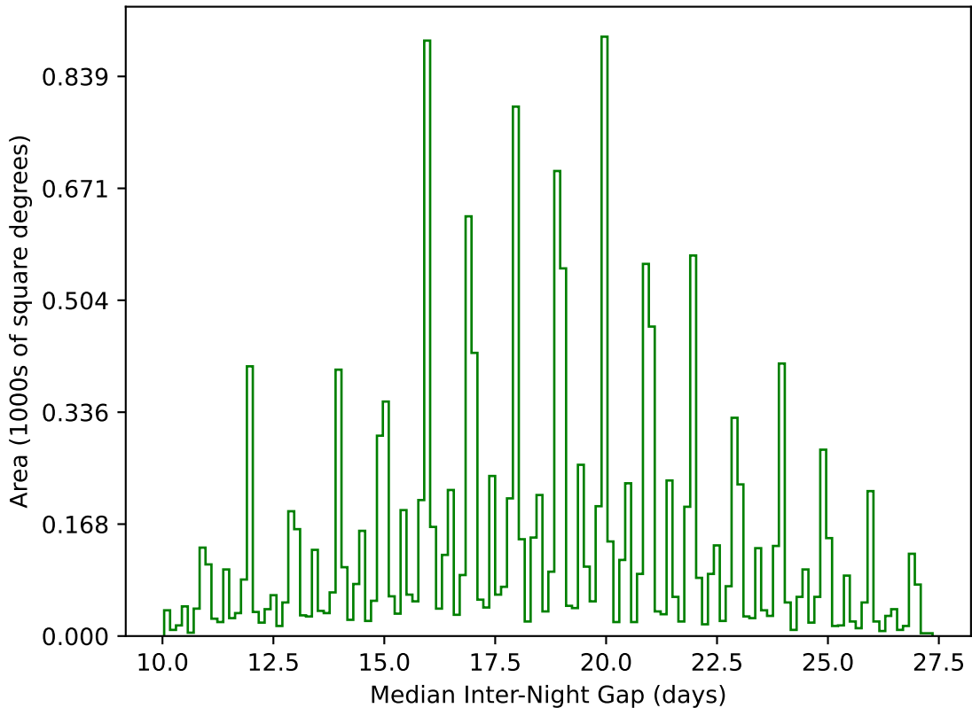
too_elab_r32_d3_uigrzy_v3.4_10yrs WFD g band: Median Inter-Night Gap
