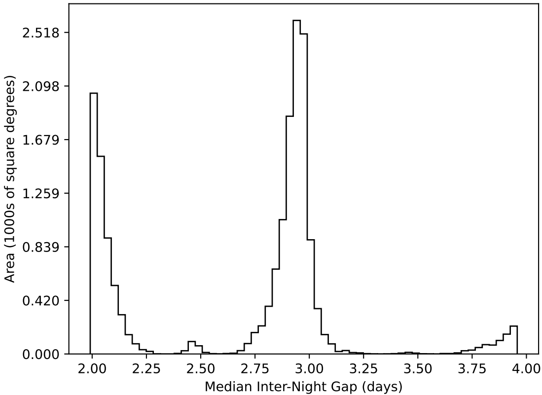
too_elab_r32_d3_ugrizy_v3.4_10yrs WFD all bands: Median Inter-Night Gap
