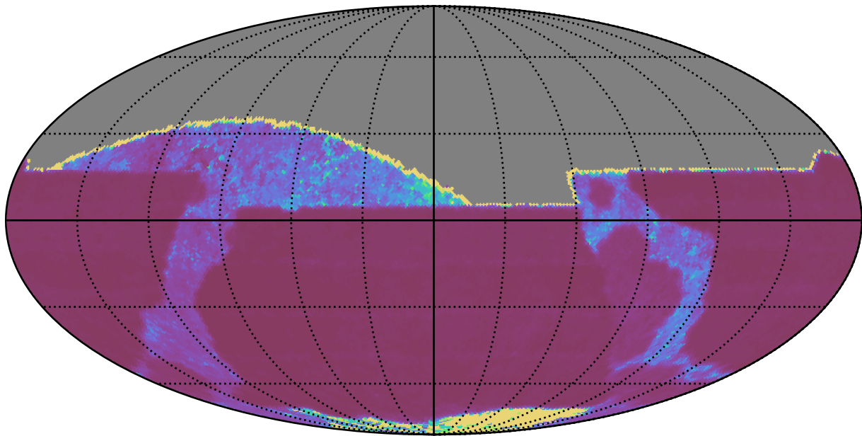
too_elab_r32_d3_ugrizy_v3.4_10yrs All sky z band: Median Inter-Night Gap
