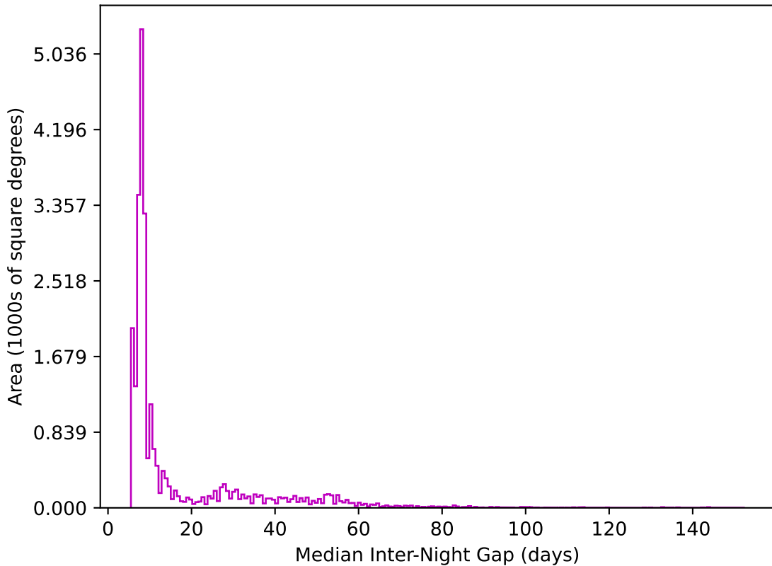
too_elab_r32_d3_ugrizy_v3.4_10yrs All sky z band: Median Inter-Night Gap
