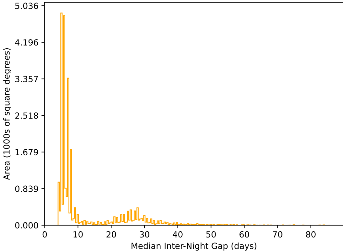
too_elab_r32_d3_ugrizy_v3.4_10yrs All sky r band: Median Inter-Night Gap
