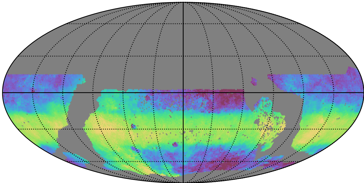
too_elab_r32_d3_ugrizy_v3.4_10yrs WFD y band: Median HA
