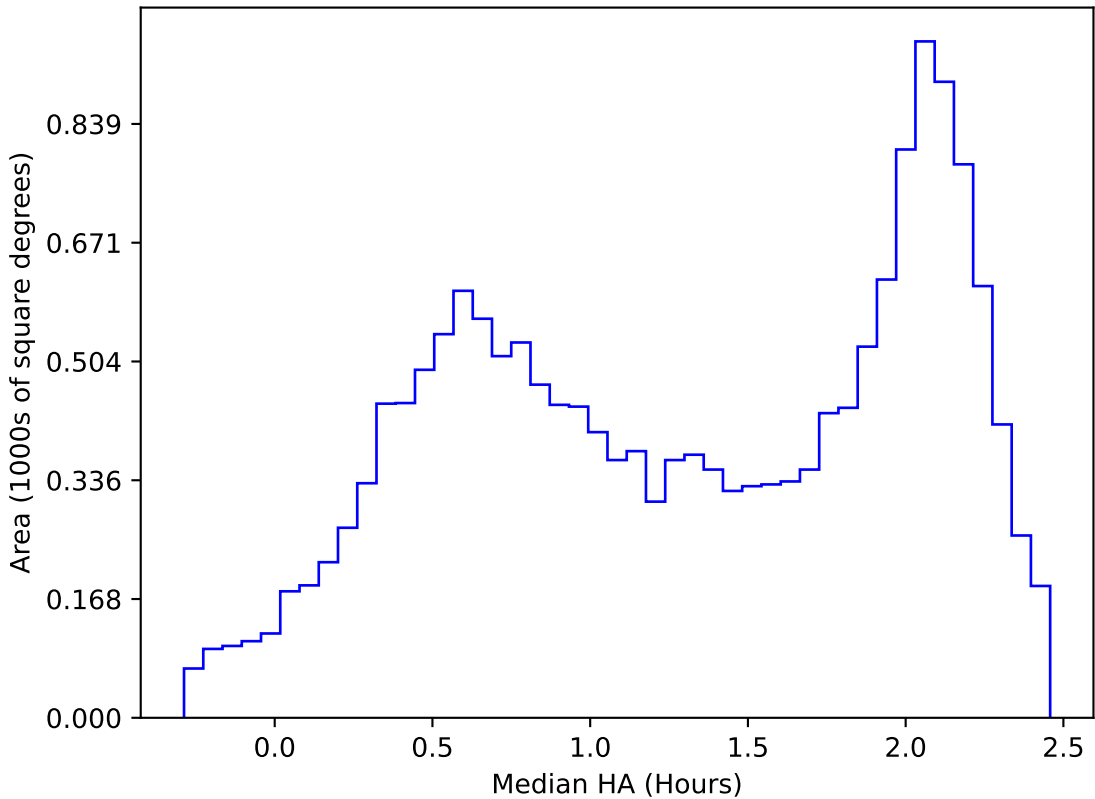
too_elab_r32_d3_ugrizy_v3.4_10yrs WFD y band: Median HA
